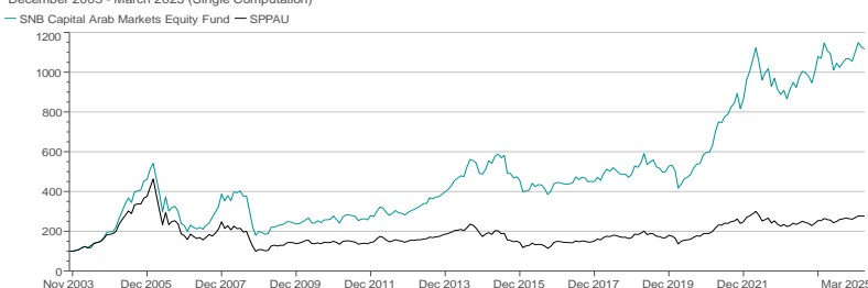
Manager Performance December 2003 - March 2025 (Single Computation)
