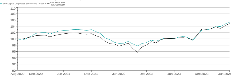
Manager Performance September 2020 - June 2024 (Single Computation)
