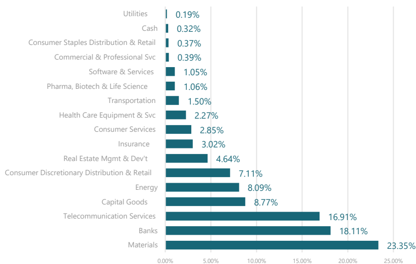
Sector Allocation
