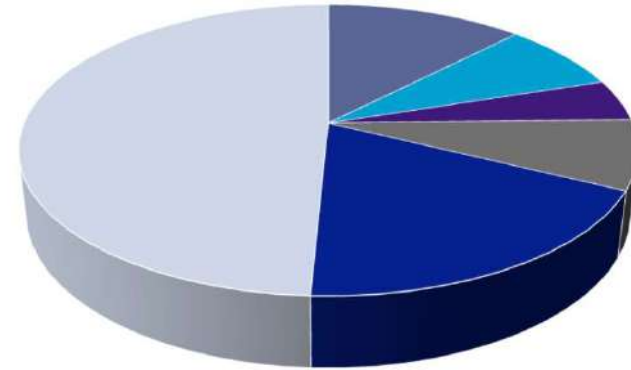
STAFF MATRIX
